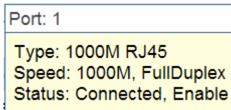
Figure 4-2 Port Information
